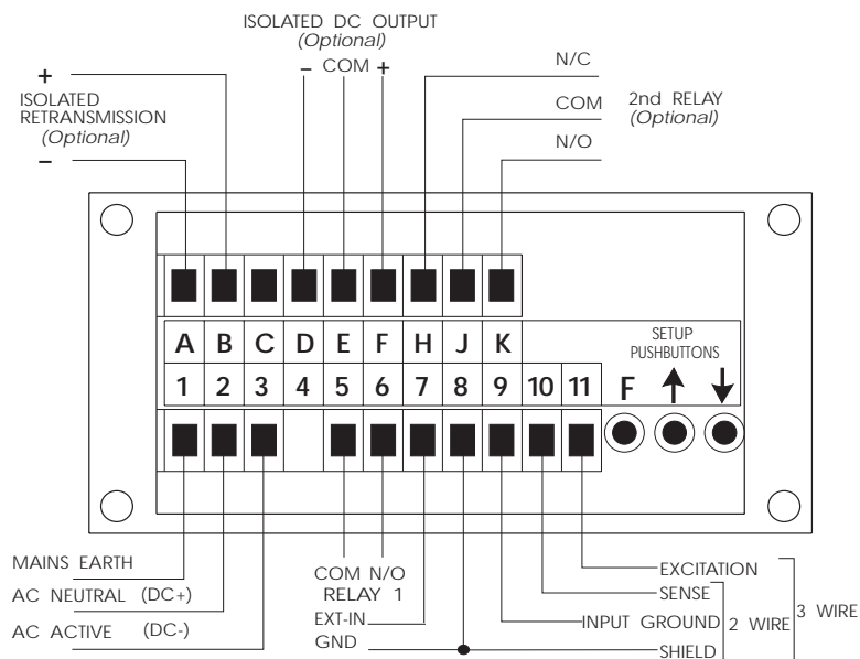
Instrument Rear Panel
